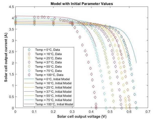
Fig. 4. Simulation of the initial parameters with experimental values (Data)
