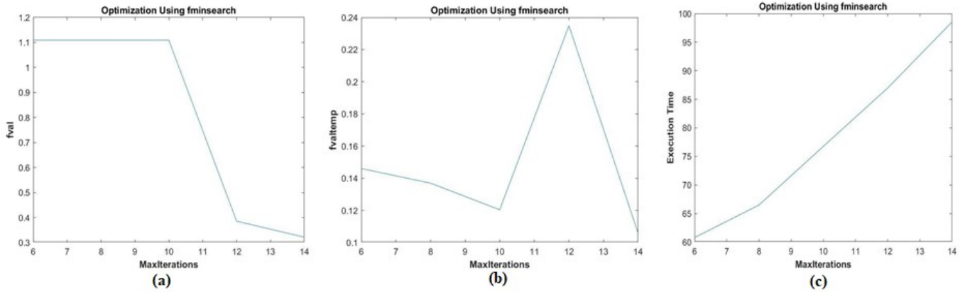
Fig. 8. Fminsearch method for (a. The fitness function value, b. The fitness function value temperature, c. Execution time)
