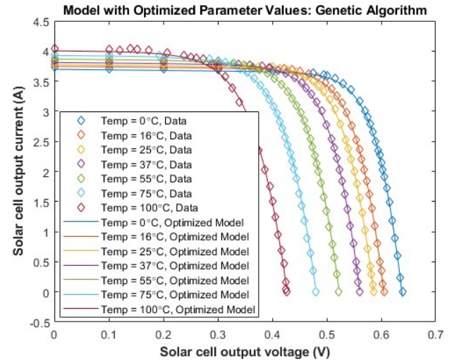
Fig. 6. Simulation of the optimization result by GA method
