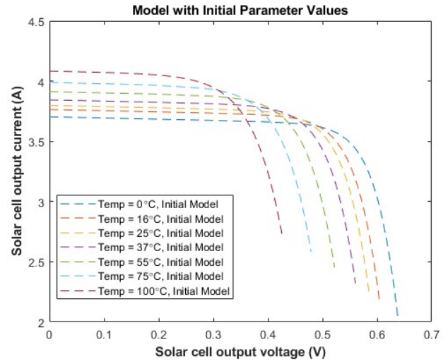
Fig. 3. Simulation of the Model with Initial Parameter Values
