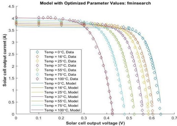
Fig. 5. Simulation of the optimization result by fminsearch method
