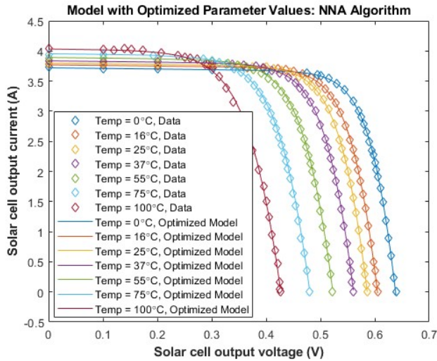
Fig. 7. Simulation of the optimization result by NNA method
