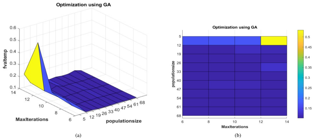
Fig. 9. (a) The fitness function temperature value using GA algorithm.(fvaltemp), (b) Selected population size of fvaltemp
