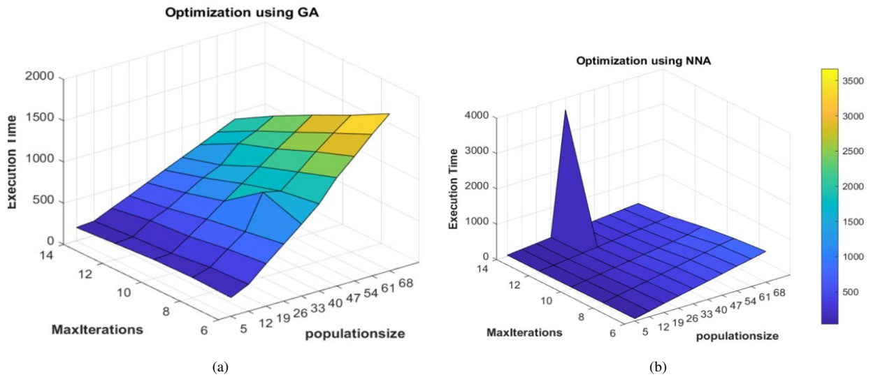
Fig. 12. the execution time for GA and NNA methods. (a) execution time for GA, (b) execution time for NNA).
