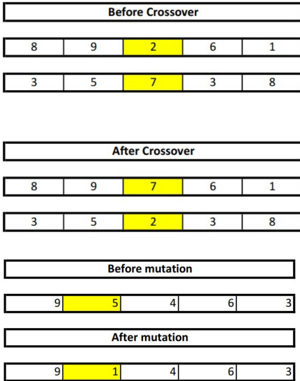
Fig. 2. Generating of chromosomes
