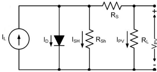
Fig. 1. Equivalent circuit of PV module [25]
