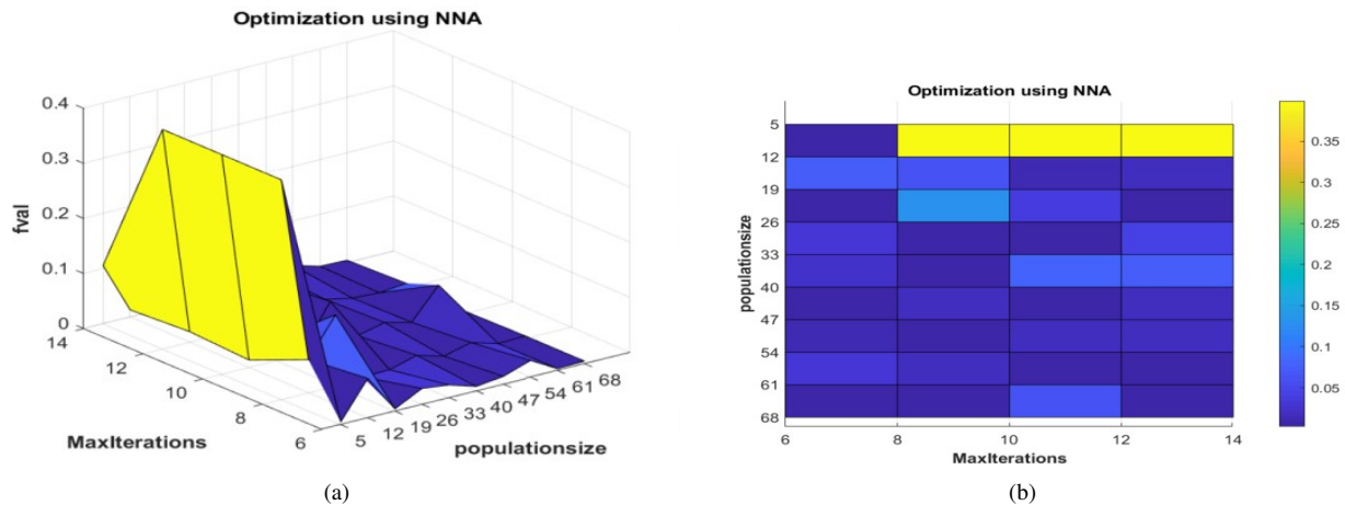
Fig. 10. (a) The fitness function value using NNA algorithm, (b) Selected population size in NNA of fval.
