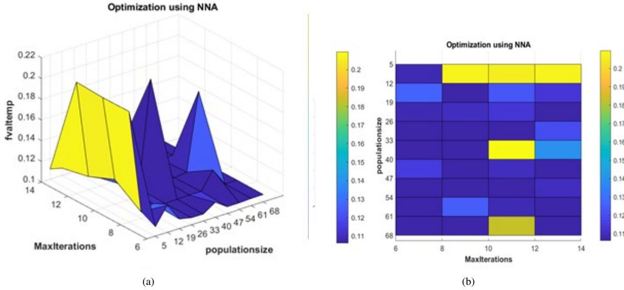
Fig. 11. (a) The fitness function temperature value using NNA algorithm, (b) Selected population size in NNA of fvaltemp
