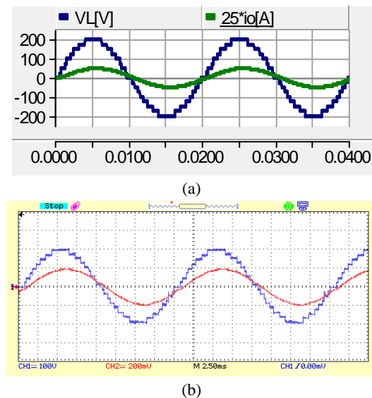
Fig. 11. Current and voltage waveforms of the load in the 17-level proposed inverter; (a) simulation result; (b) experimental result.
