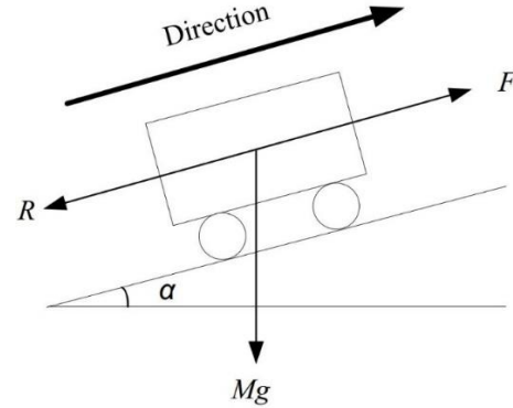
Fig. 1: Forces on a traction vehicle
