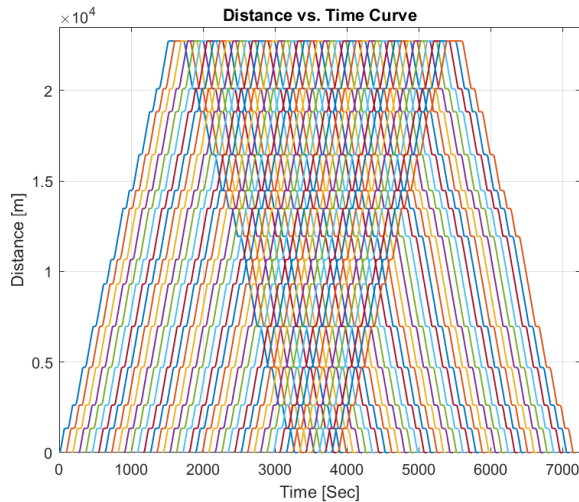
Fig. 19: Trains location vs. time
