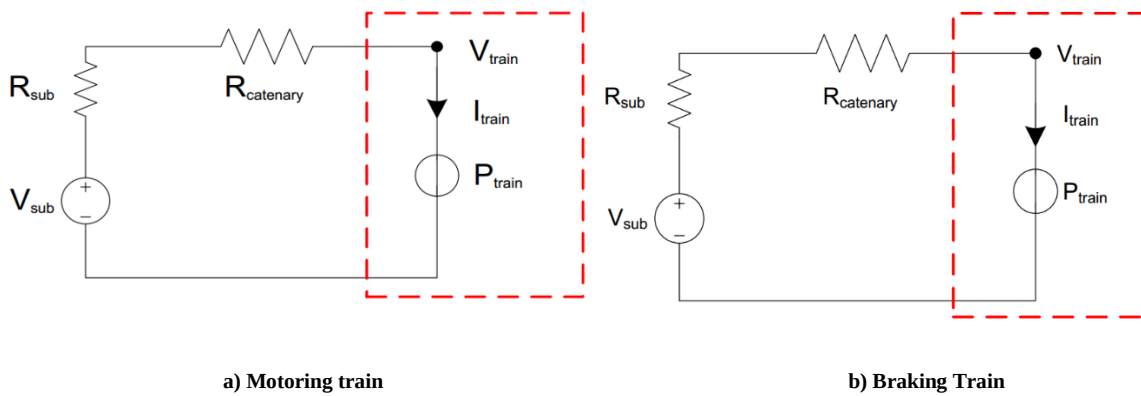
Fig. 9: Equivalent model Train
