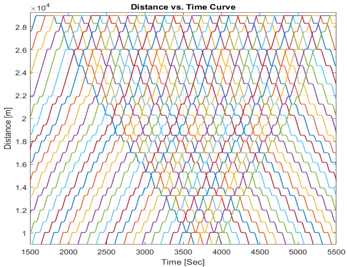
Fig. 22: The movement timetable of trains in TML2
