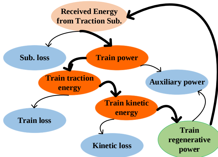
Fig. 5: The power flow diagram in the railway system
