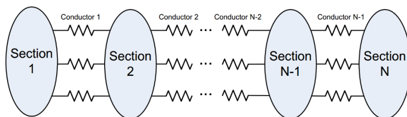
Fig. 11: Chain circuit topology of railway equivalent circuit
