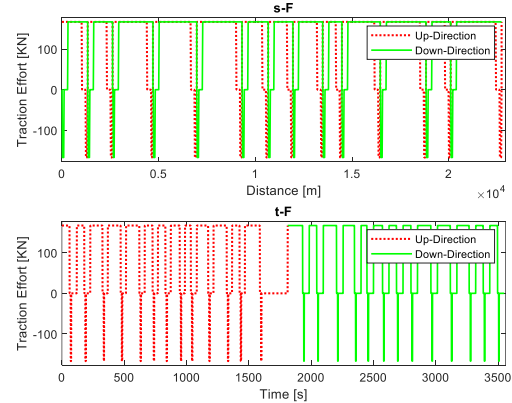
Fig. 16: Train tractive effort vs. location and time in both up and down directions
