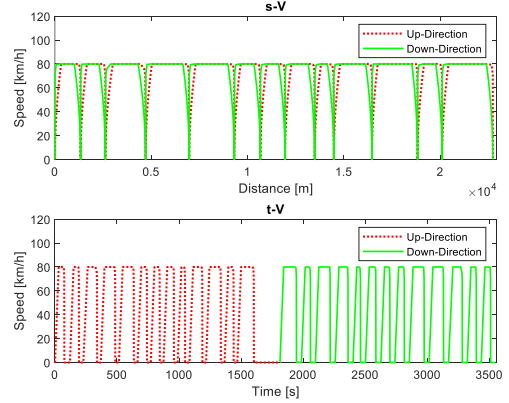
Fig. 15: Train speed vs. location and time in both up and down directions
