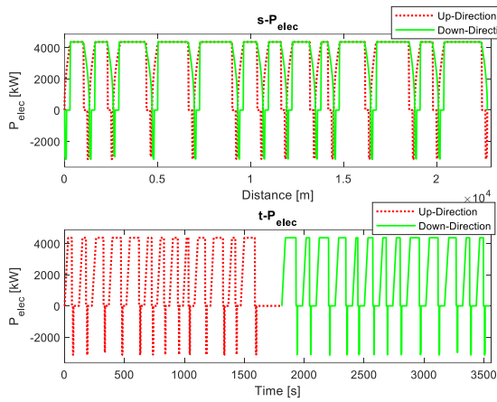
Fig. 18: Train P_{elec} vs. location and time in both up and down directions
