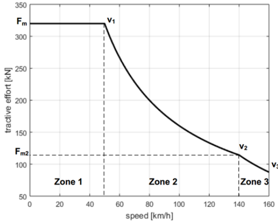
Fig. 2: Tractive effort curve of a suburban train
