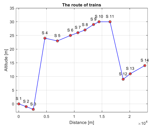
Fig. 12: Route vertical alignment and train station location
