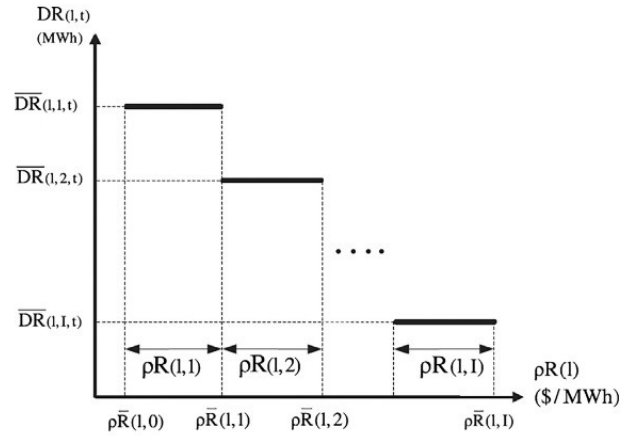
Fig. 2. Price-load curve of the demand supplied by the retailer [33]
