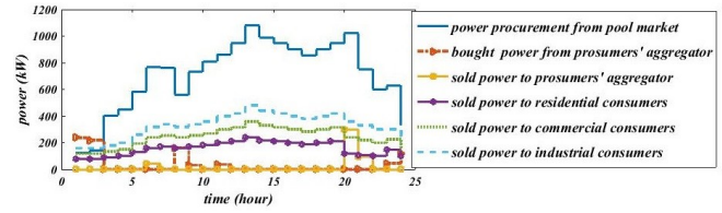
Fig. 9. The power procurement of the retailer in FP method (case 2a)
