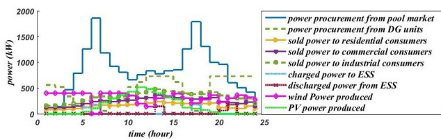
Fig. 8. The power procurement of retailer and prosumers' aggregator in case 1
