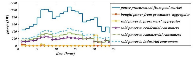
Fig. 11. The power procurement of the retailer in TOU method (case 2b)
