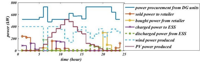
Fig. 10. The power procurement of the prosumers' aggregator in FP method (case 2a)
