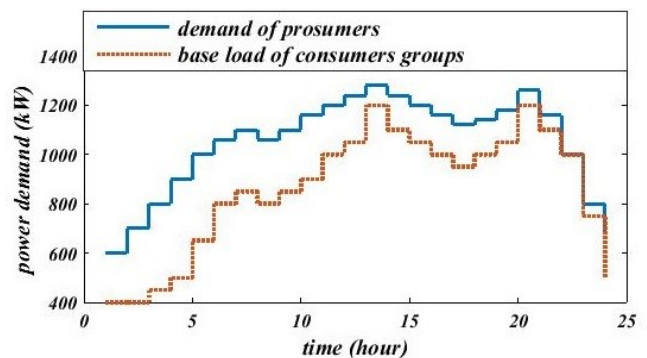
Fig. 7. Base load profile for retailer's consumers group and demand profile of the prosumers' aggregator
