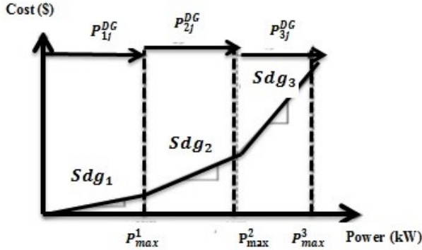
Fig. 3. Linear operation cost model of DG units [33].
