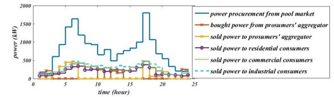
Fig. 13. The power procurement of the retailer in RTP (case 2c)
