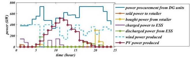
Fig. 12. The power procurement of the prosumers' aggregator in TOU method (case 2b)
