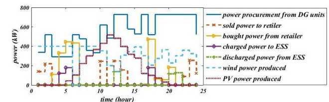
Fig. 14. The power procurement of the prosumers' aggregator in RTP method (case 2c)
