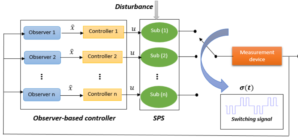
Fig. 1. Closed-loop system operation
