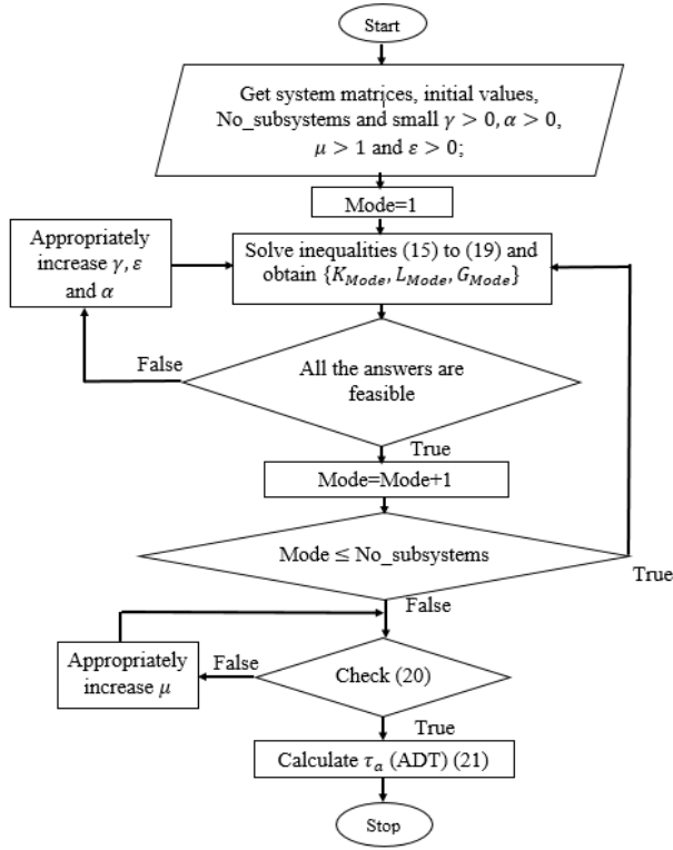
Fig. 2. H_\infty observer-based design flowchart
