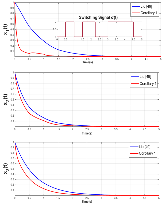
Fig. 13. Three states convergence with both methods
