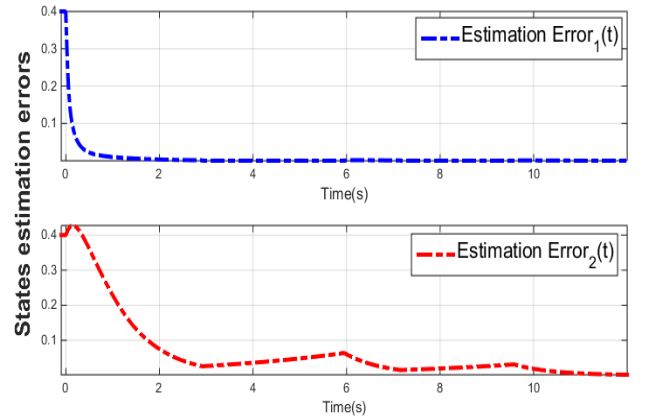
Fig. 6. Error signal for 12 seconds running time
