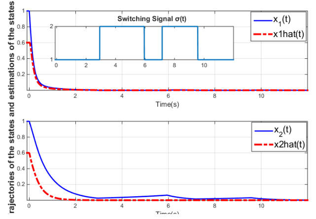
Fig. 5. State trajectories and estimation
