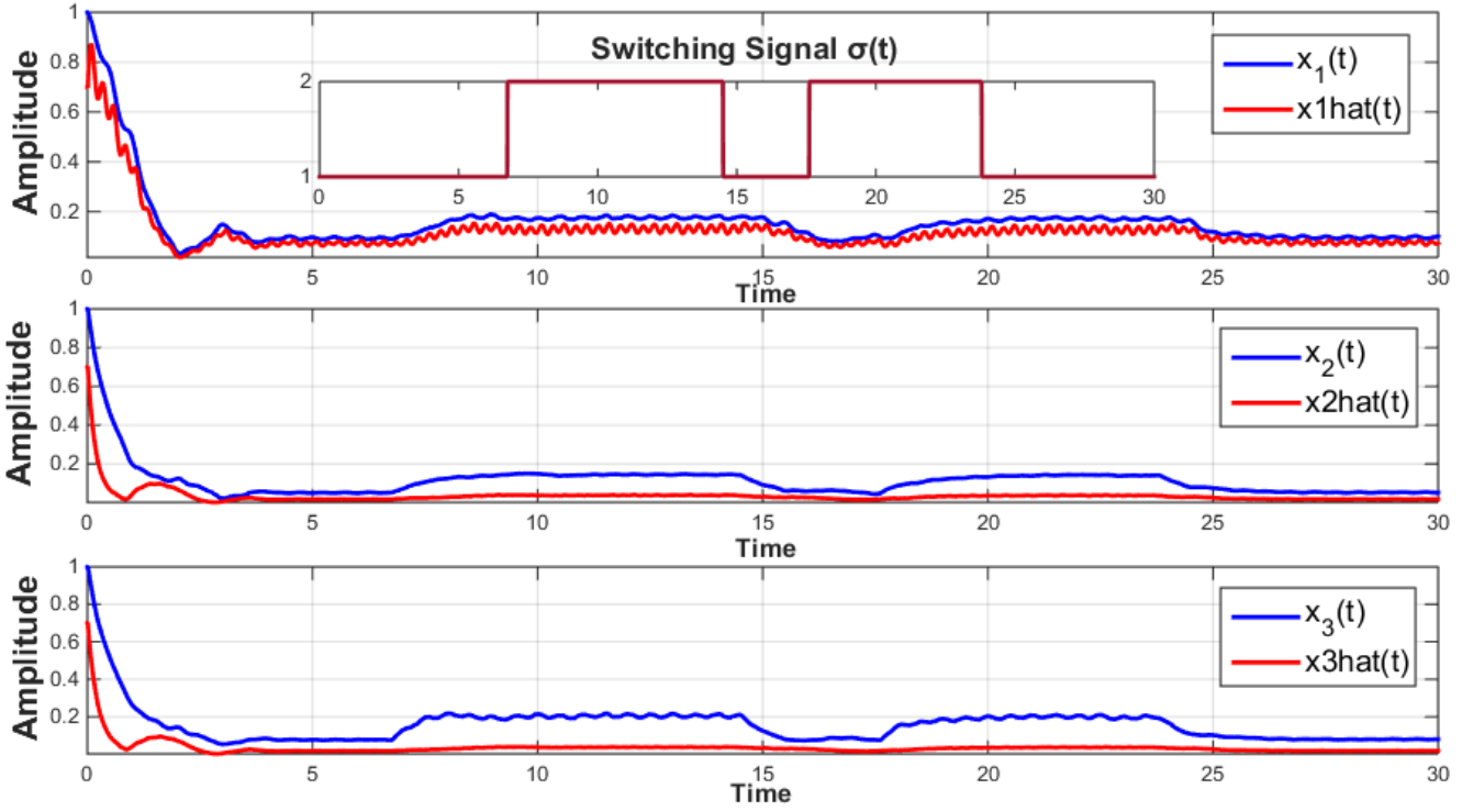
Fig. 12. States and their estimations
