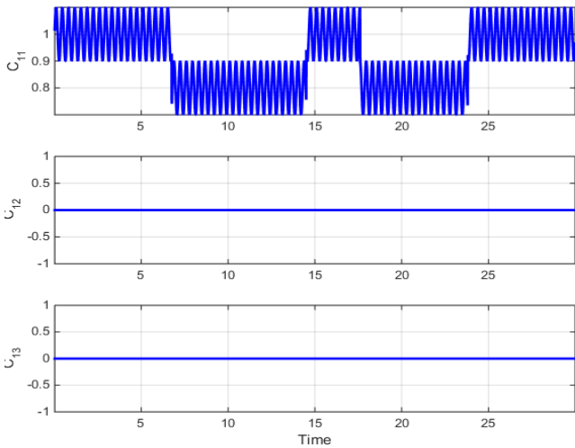
Fig. 11. Parameter uncertainties of A matrix elements
