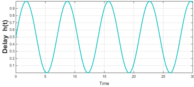
Fig. 9. Time-varying delay for case no. 2
