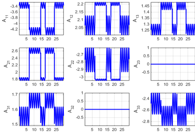
Fig. 10. Parameter uncertainties of A matrix elements
