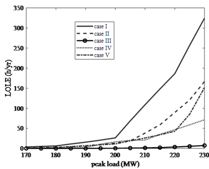
Fig. 9. LOLE at different peak demand.
