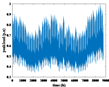
Fig. 11. Hourly peak load in per unit.
