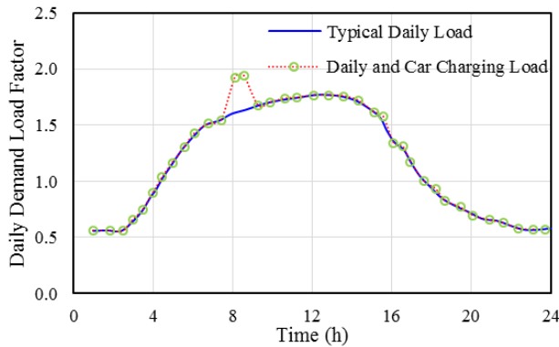
Fig. 4. Typical load and car charging effect on daily load demand.
