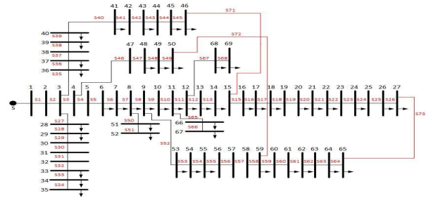
Fig. 7. SLD of IEEE-69 bus RDS with network reconfiguration.
