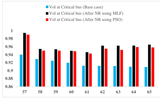
Fig. 9. Comparison of voltage magnitudes at critical buses before and after NR of 69 bus RDS.
