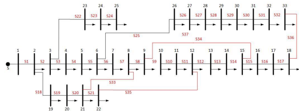
Fig. 3. SLD of IEEE-33 bus RDS with network reconfiguration.
