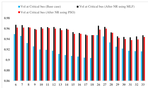
Fig. 5. Comparison of voltage magnitudes at critical buses before and after NR of 33 bus RDS.
