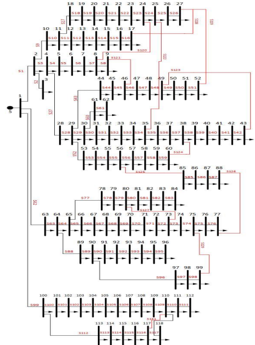
Fig. 11. SLD of IEEE-118 bus RDS with network reconfiguration.
