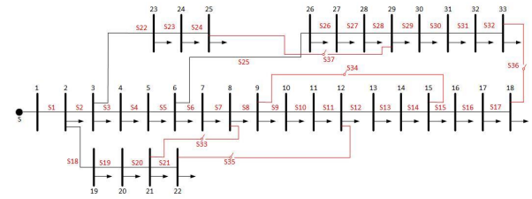
Fig. 2. SLD of IEEE-33 bus RDS.
