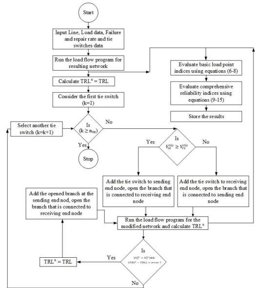
Fig. 1. Flow chart for MLF for NR of RDS for minimization of TRL.
