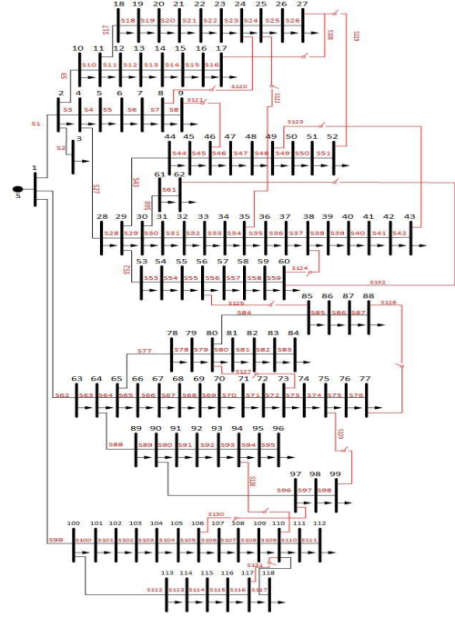
Fig. 10. SLD of IEEE-118 bus RDS.
