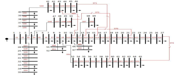
Fig. 6. SLD of IEEE-69 bus RDS.
