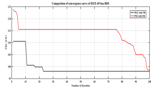
Fig. 8. Comparison of convergence curves of 69 bus RDS.
