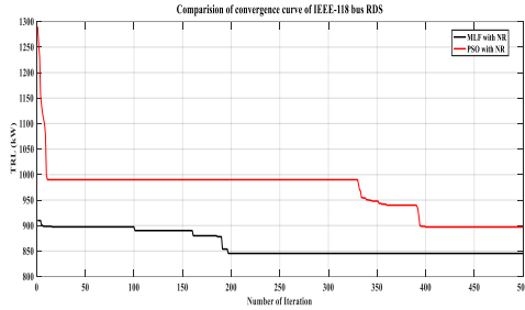
Fig. 12. Comparison of convergence curves of 118 bus RDS.
