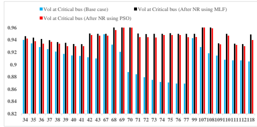
Fig. 13. Comparison of voltage profiles at critical buses without and with NR of IEEE-118 bus RDS.
