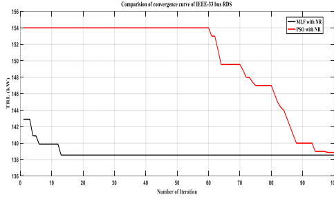
Fig. 4. Comparison of convergence curves of IEEE-33bus RDS.
