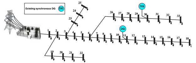
Fig. 1. Single-line diagram of the 33-bus test system.
