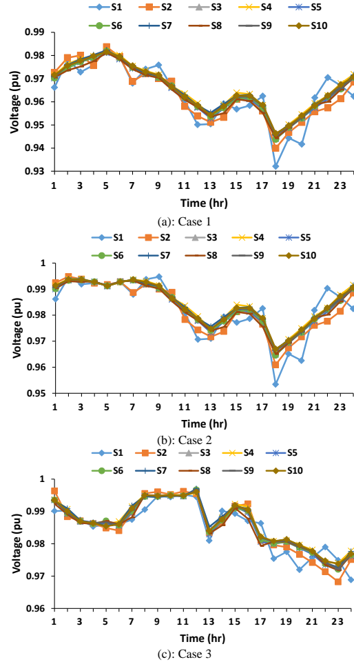
Fig. 9. Voltage magnitude of bus 18 in three cases under different uncertainty scenarios.
