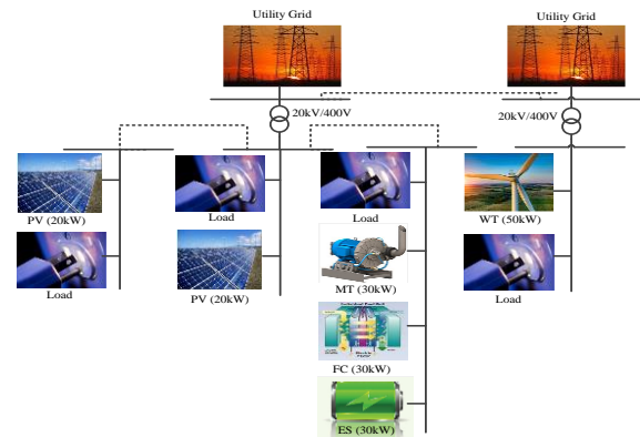
Fig. 1. The studied microgrid [36]
